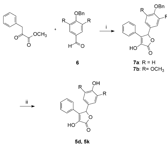
Scheme 2. Reagents and conditions: (i) DBU, DMF, 0^\circ C ; (ii) Pd/C, H_2 , EtOH/THF.
