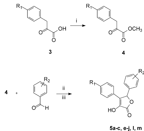
Scheme 1. Reagents and conditions: (i) DBU, CH_3I , DMF, 0^\circ C ; (ii) DBU, DMF, 0^\circ C ; (iii) HCl.
