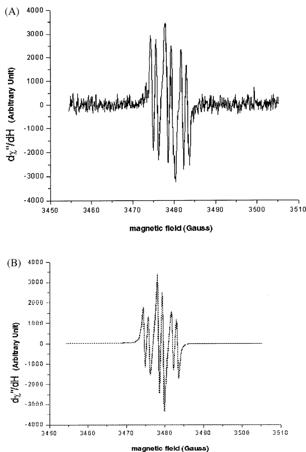
Figure 1. ESR spectrum of stable semiquinone radical generated from compound 5g . (A) Experimental spectrum recorded after NaOH addition. Spectrometer setting: microwave power, 10 mW, modulation amplitude, 0.5 gauss, scan range, 100 gauss, frequency, 9.42 GHz. (B) Simulated ESR spectrum.
